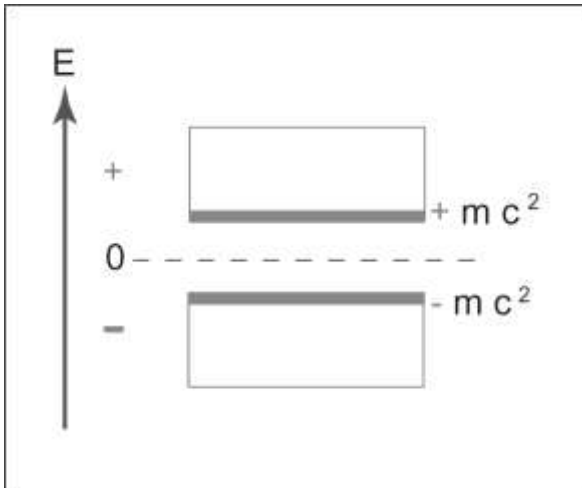
Figure 1. Schematic energy spectrum associated with the Dirac Equation.
